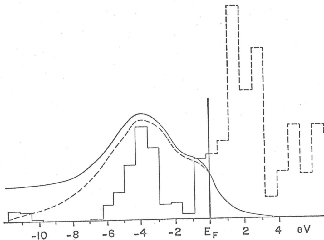
FIG. 15. Nb-L III emission from NbC.
