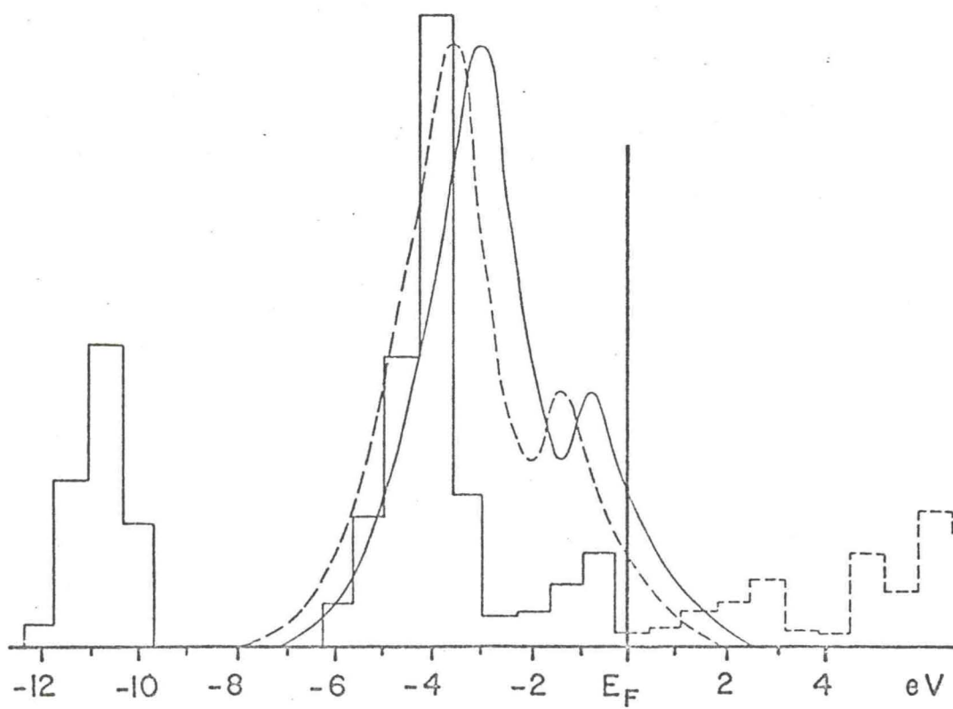
FIG. 16. Nb-Ni IV,V emission from NbC.
